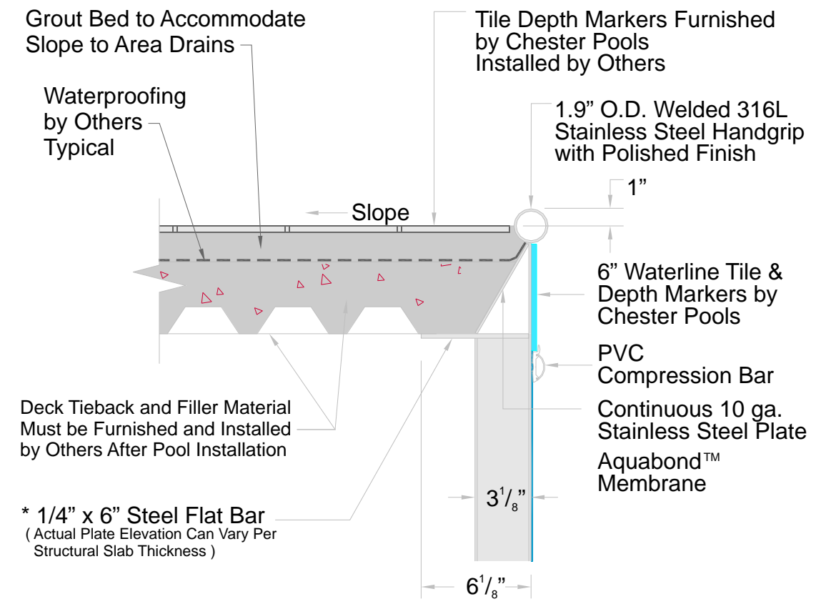
Bullnose Coping Section Detail
